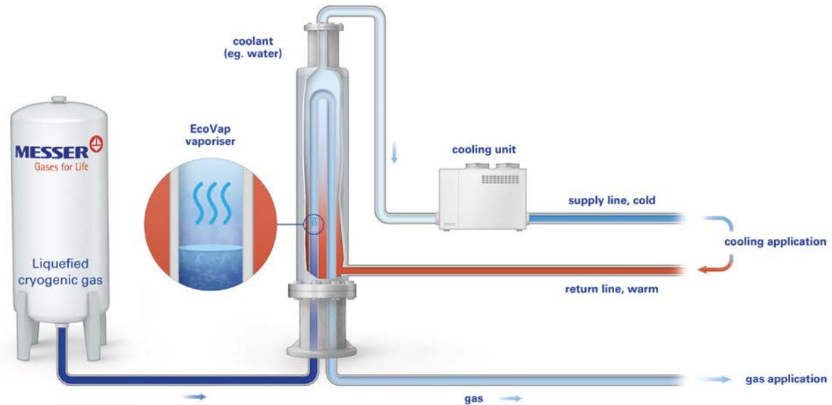
Principle of EcoVap vaporiser process
